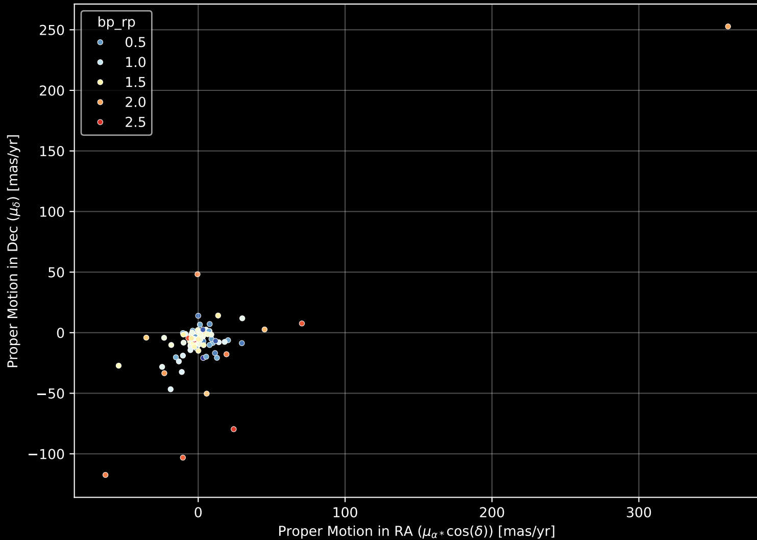
APOGEE DR17 Field: [047-25_MGA] Proper Motion Diagram (n= 128)
