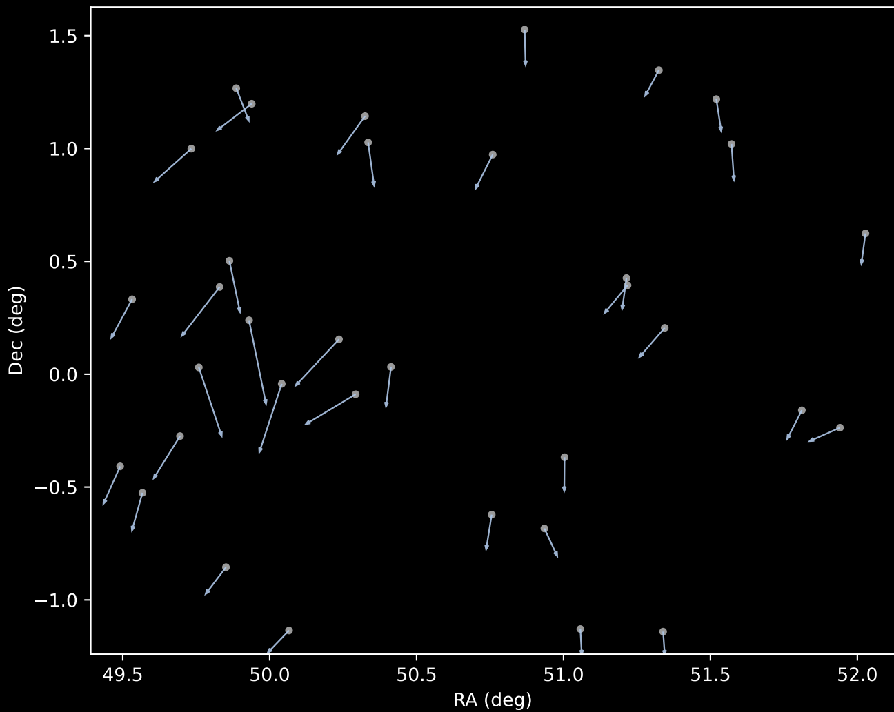
APOGEE DR17 Cluster 1 Proper Motion Vectors (n=35)
