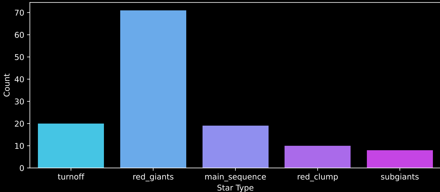
APOGEE DR17 Field: [047-25_MGA] Count plot of Star Type
