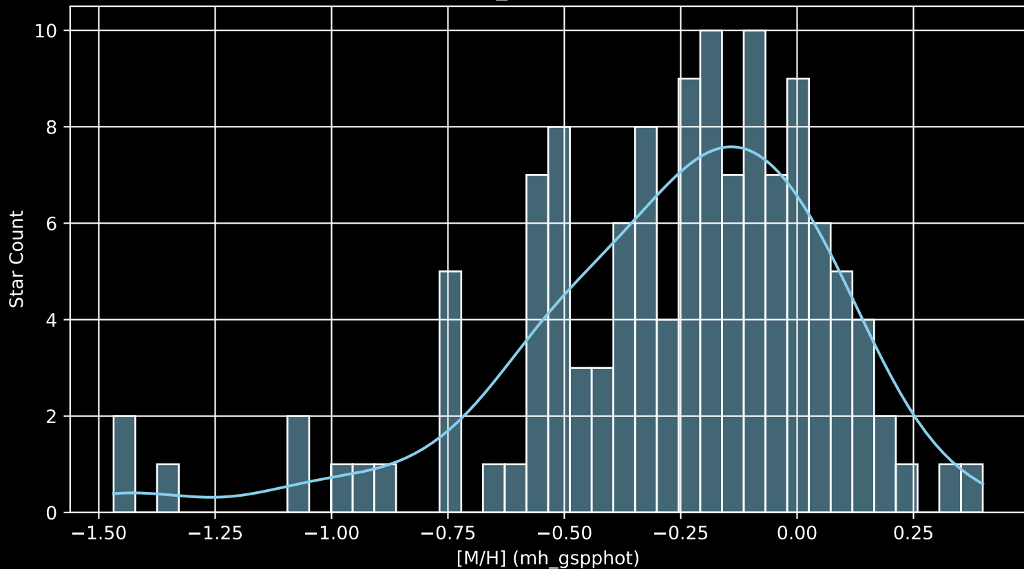
APOGEE DR17 Field: [047-25_MGA [M/H] (mh_gspphot) (n= 126)
