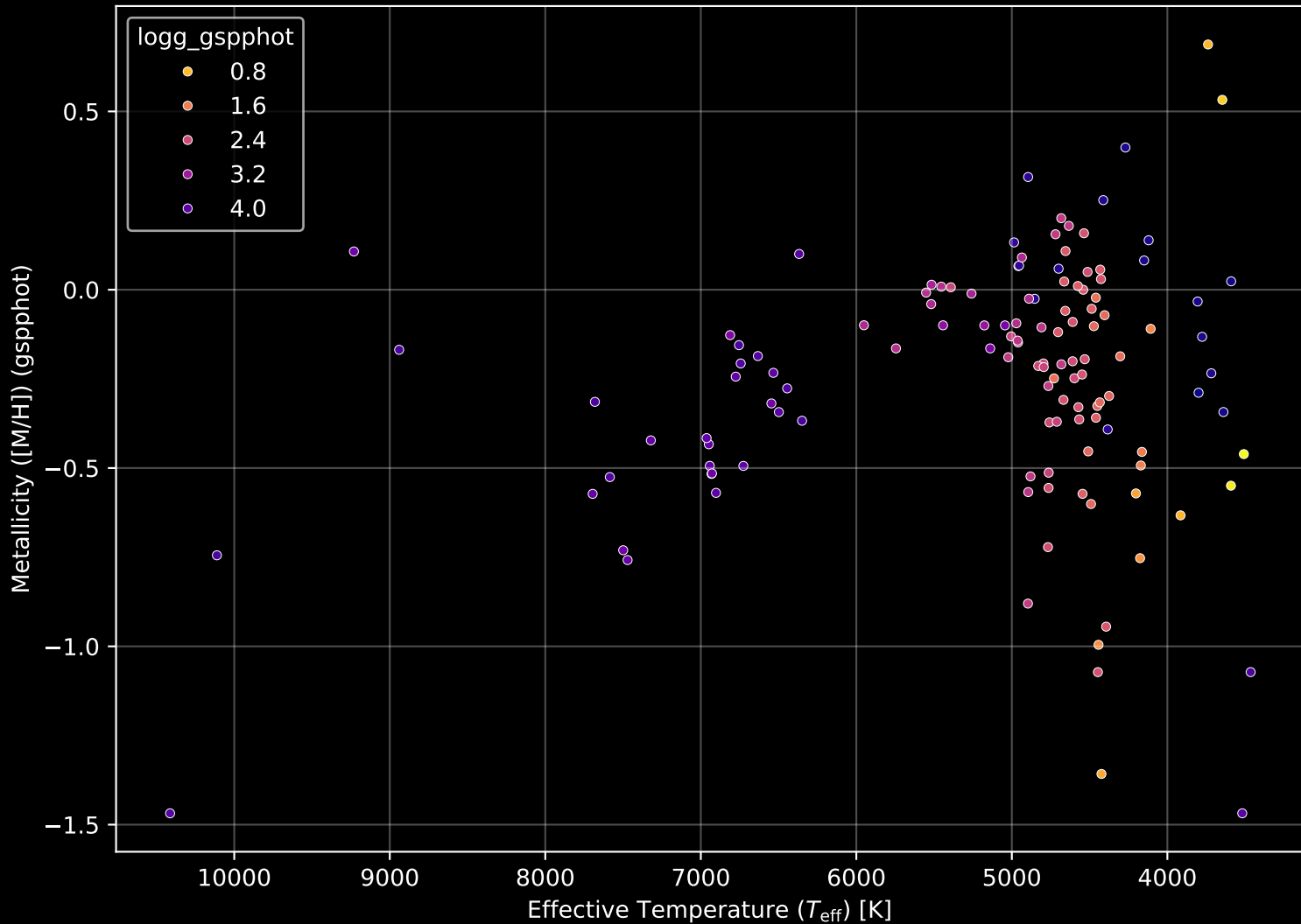
APOGEE DR17 Field: [047-25_MGA] Stellar Population Parameters (n= 128)
