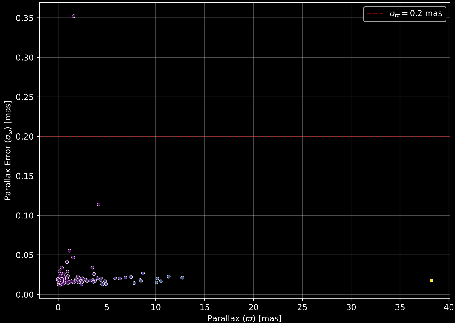
APOGEE DR17 Field: [047-25_MGA] Parallax Quality (n= 128)
