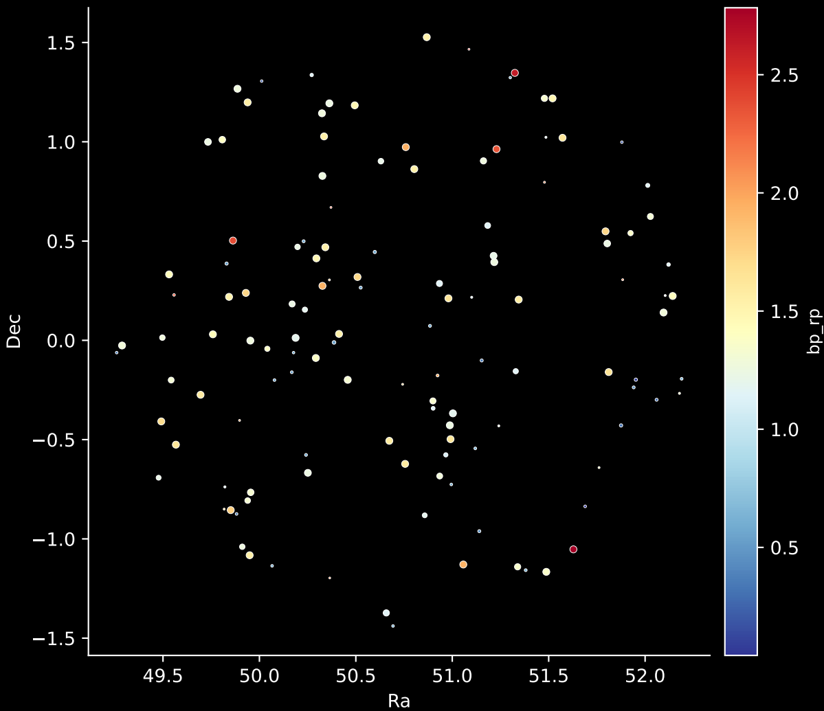
APOGEE DR17 Field: [047-25_MGA] Stars: 128
