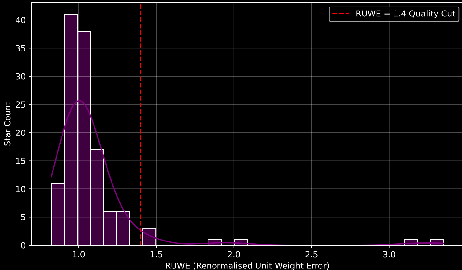
GAPOGEE DR17 Field [047-25_MGA] RUWE Distribution (n= 126)
